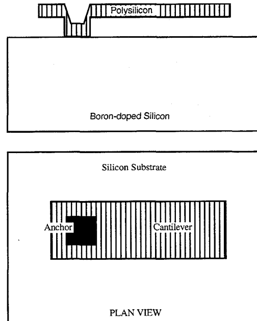
Fig. 2: Cross section and plan views of micro-cantilever
