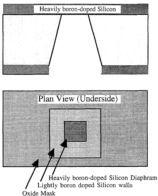
Fig. 3: Cross section and plan views of micro-diaphragm
